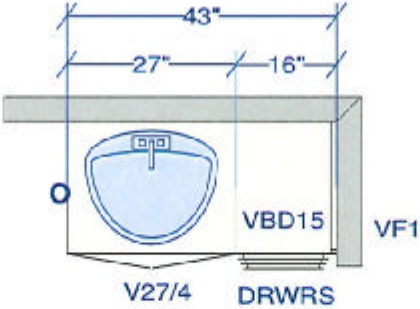
MAIN BATH
