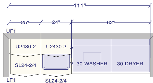
LAUNDRY ROOM
