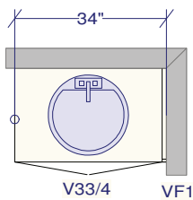
POWDER ROOM
