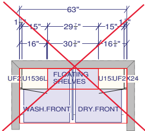
LAUNDRY CLOSET (2ND FLOOR)
