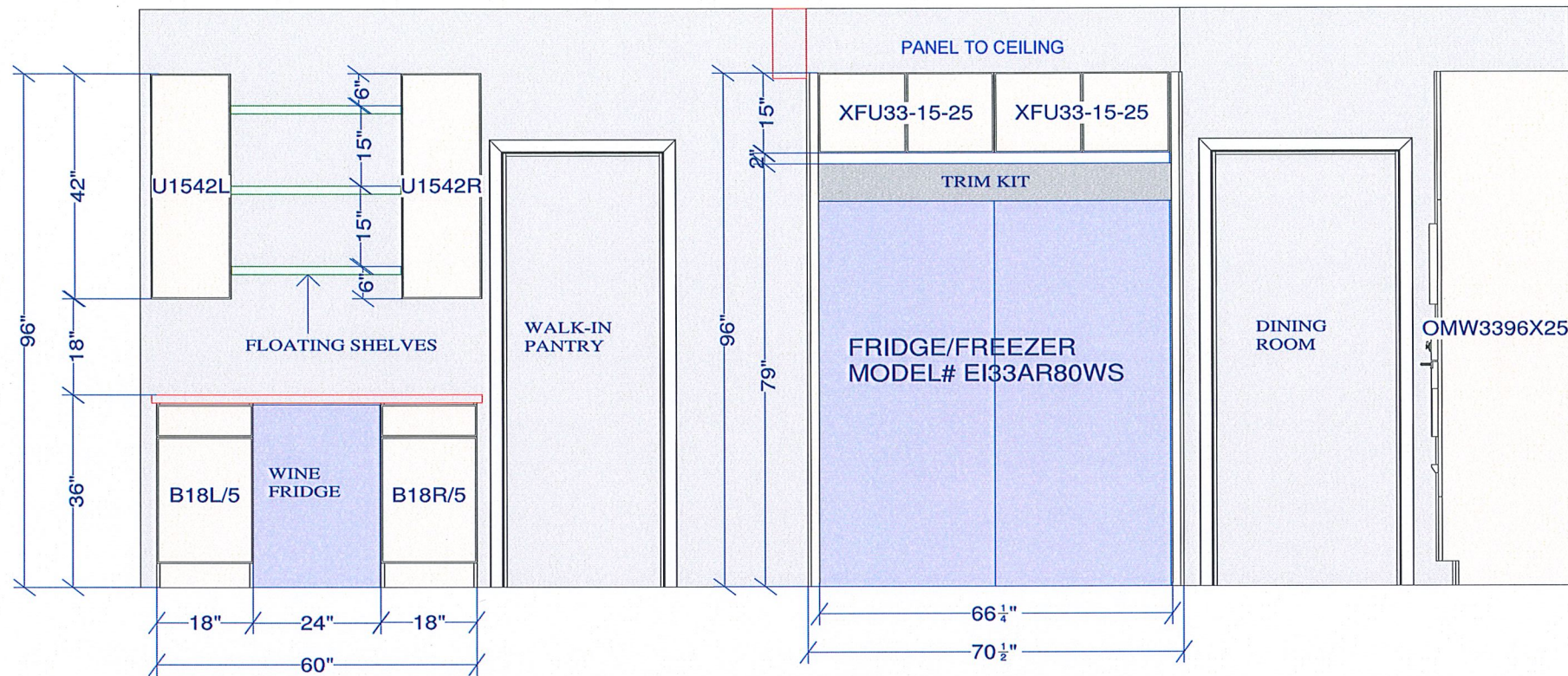
FRIDGE/FREEZER ELEVATION
