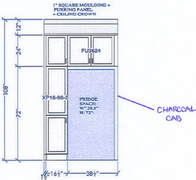
FRIDGE WALL ELEVATION
