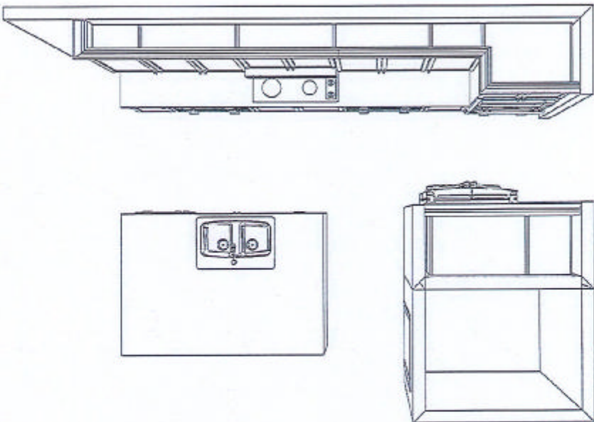
KITCHEN - TOP VIEW
