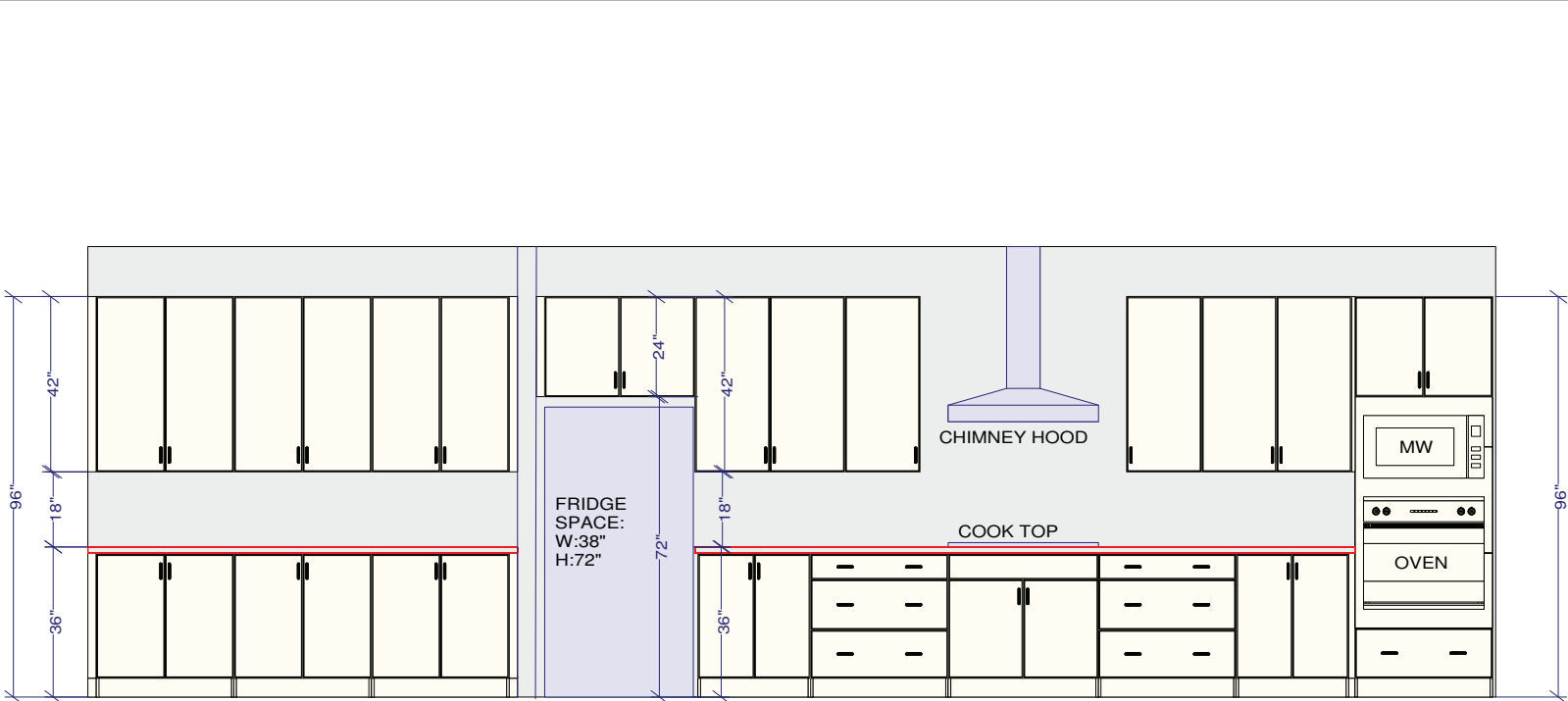
BUTLER'S PANTRY ELEVATION
