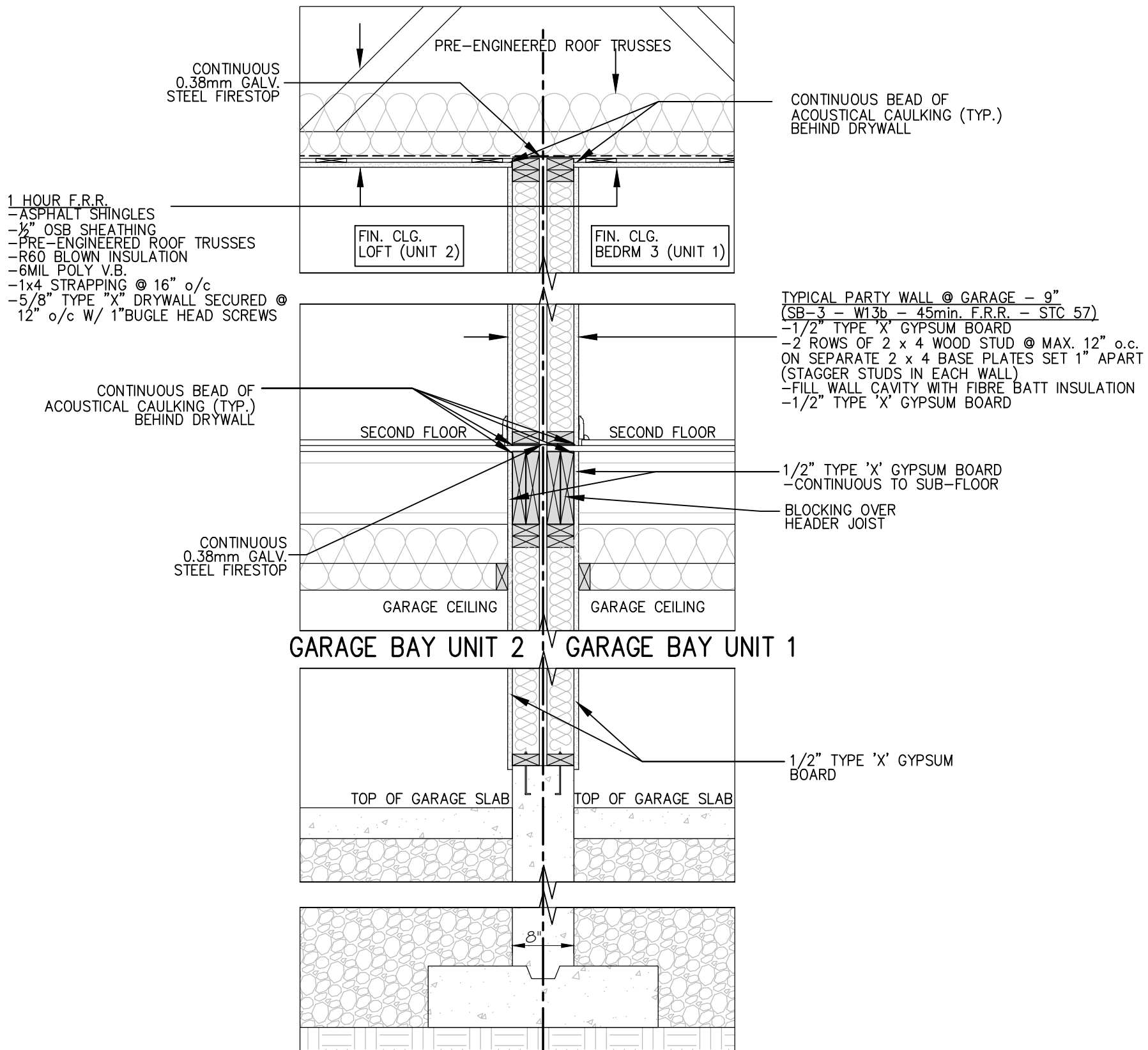
1 PARTY WALL DETAIL @ GARAGE FD-1 SCALE: 3/4"=1'
