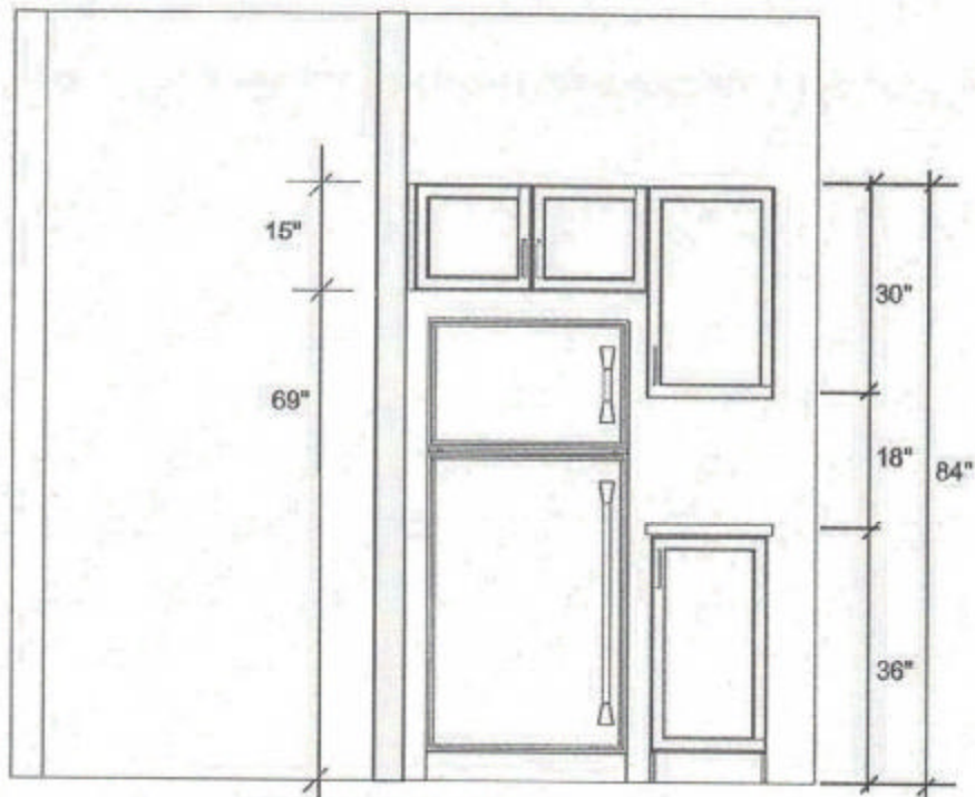
FRIDGE WALL ELEVATION KLONDIKE BASEMENT APT - 2 BDRM
