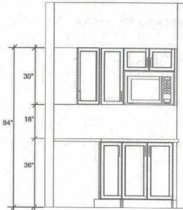
MICROWAVE WALL ELEVATION KLONDIKE BASEMENT APT - 2 BDRM
