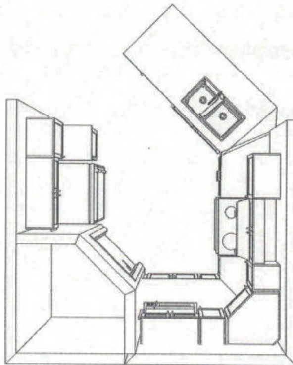
KITCHEN TOP VIEW KLONDIKE BASEMENT APT - 2 BEDROOM
