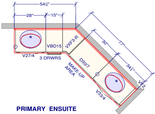
PRIMARY ENSUITE
