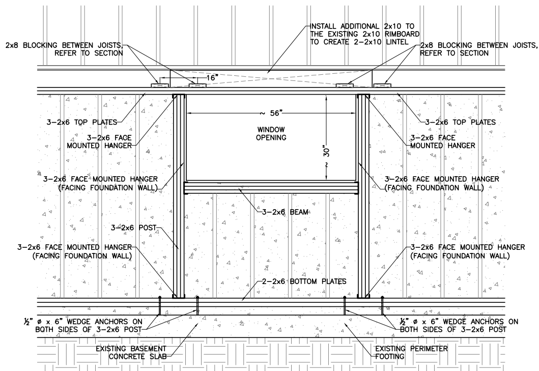
FRAMED REINFORCEMENT AROUND A LATERALLY UNSUPPORTED FOUNDATION WALL BELOW WINDOW — ELEVATION VIEW (NOT TO SCALE)
