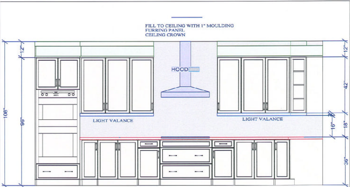
OVEN WALL ELEVATION
