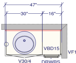
MAIN BATH
