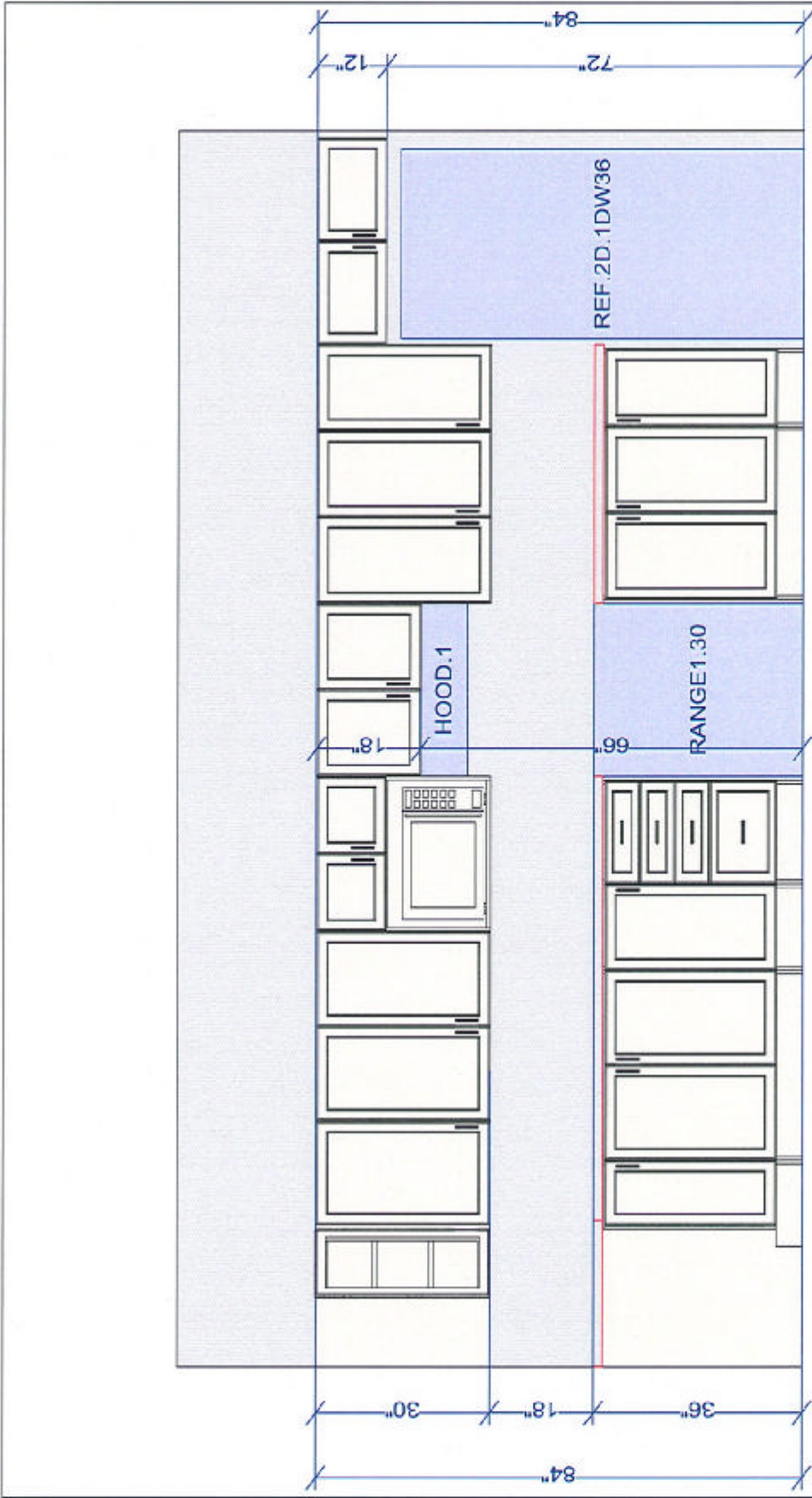
RANGE & FRIDGE WALL ELEVATION
