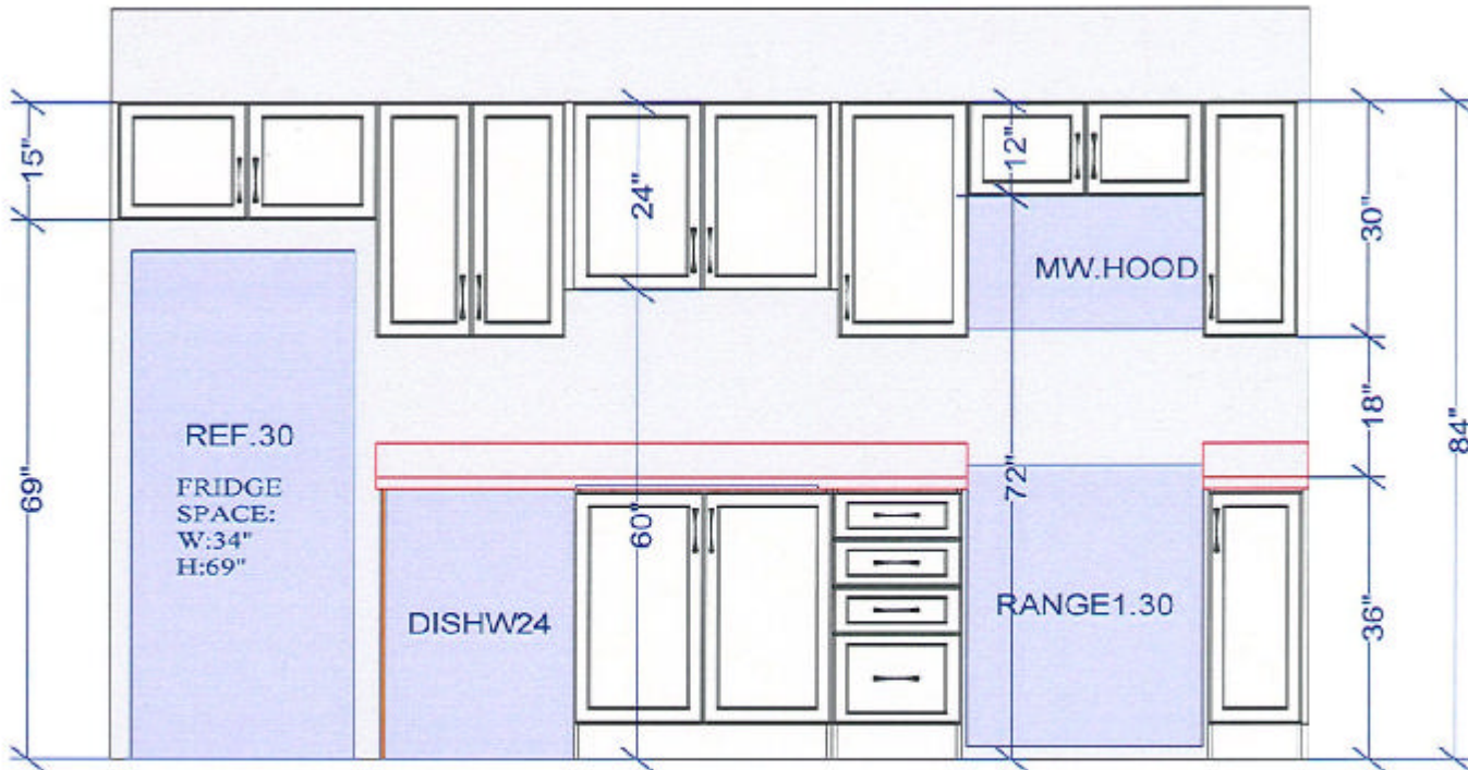
FRIDGE / RANGE WALL ELEVATION
