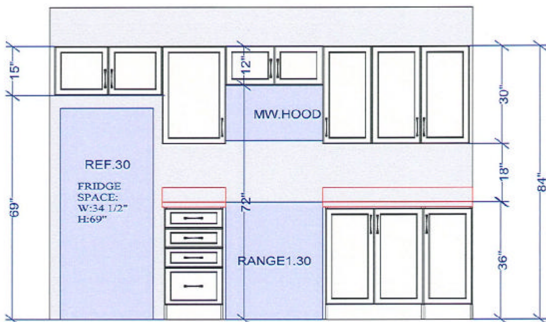
FRIDGE / RANGE WALL ELEVATION
