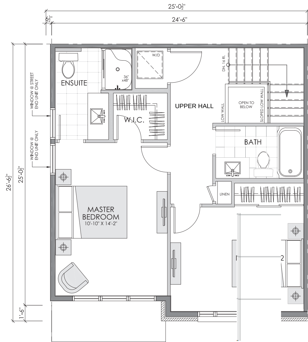
UPPER UNIT: UPPER FLOOR
