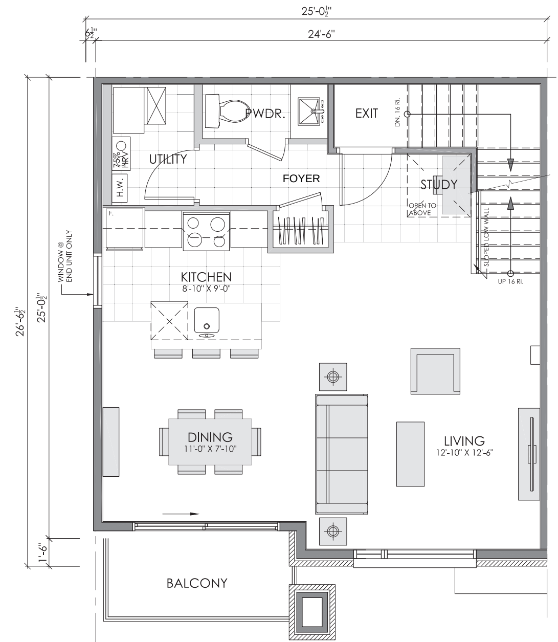
UPPER UNIT: MAIN FLOOR
