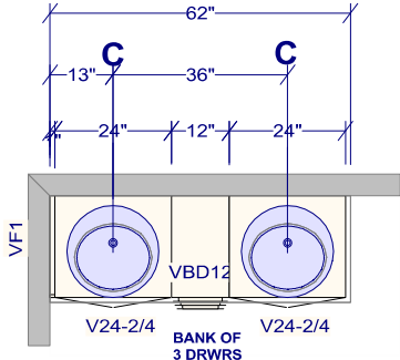
PRIMARY ENSUITE
