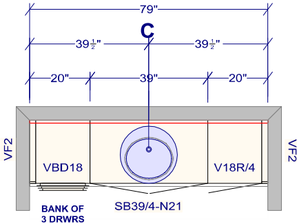
MAIN BATH
