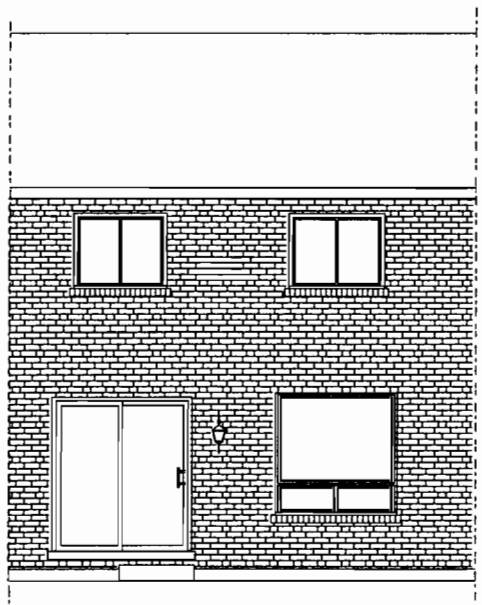
Back Elevation
