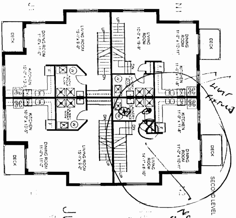
Jupiter 915 sq. ft.
