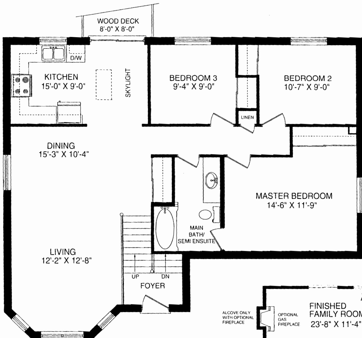
Upper Level
