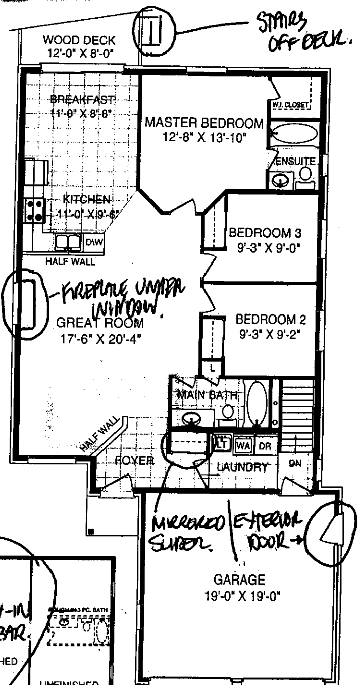
Main Floor 3 Bedroom
