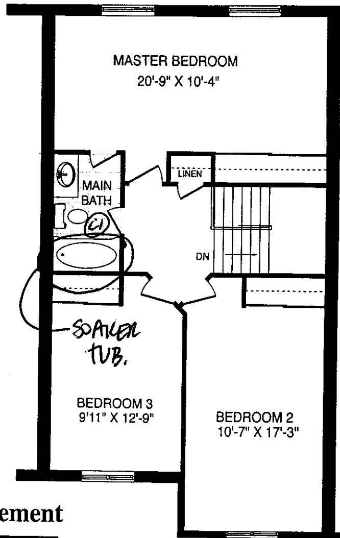
Second Floor
