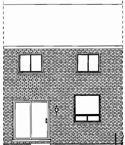
Back Elevation
