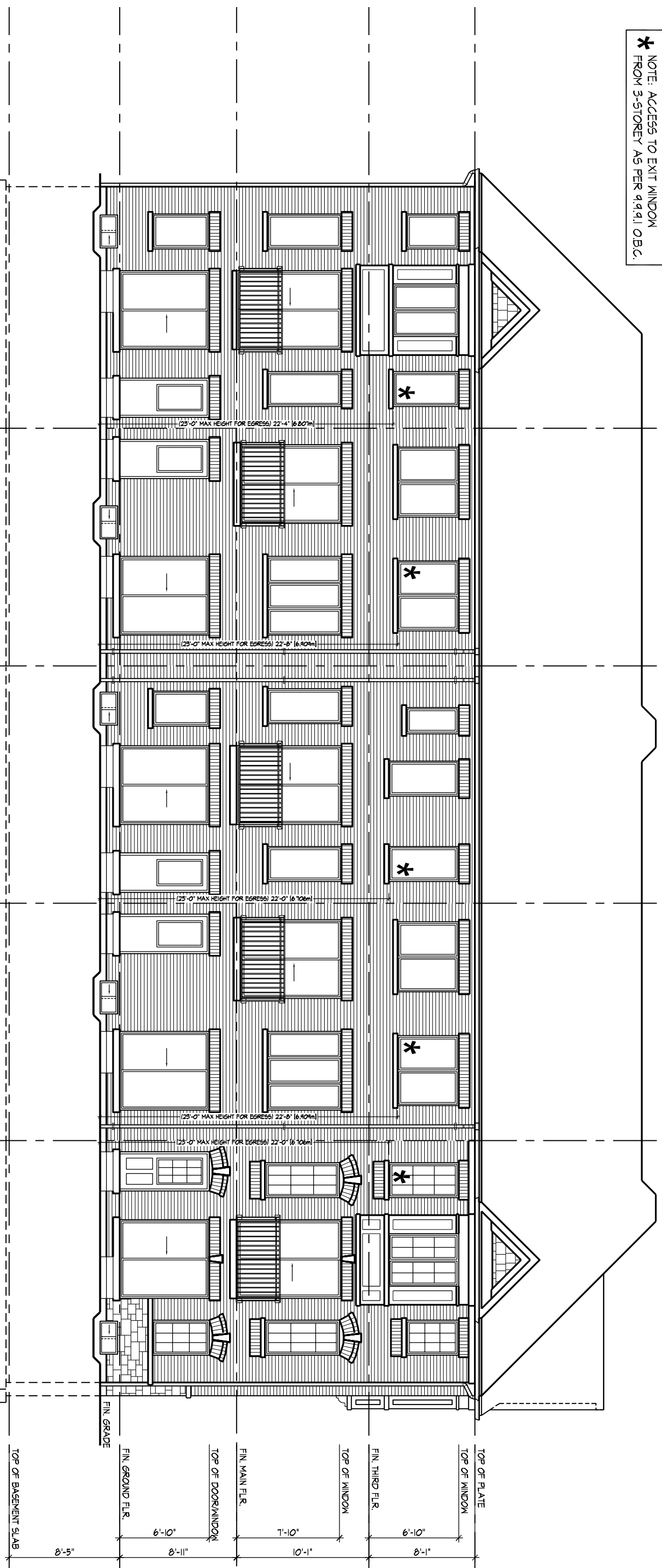
1804 E.L. "A" - CORNER FRONT ELEVATION
