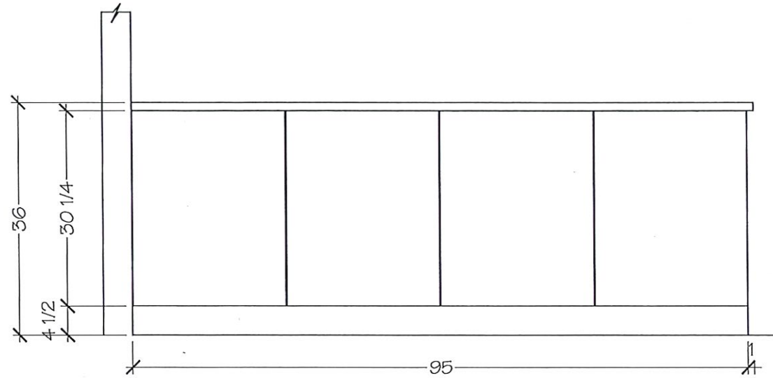
BACK ELEVATION
