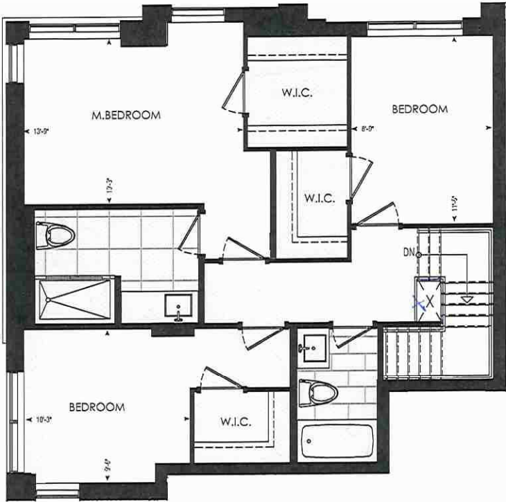
UPPER FL.
