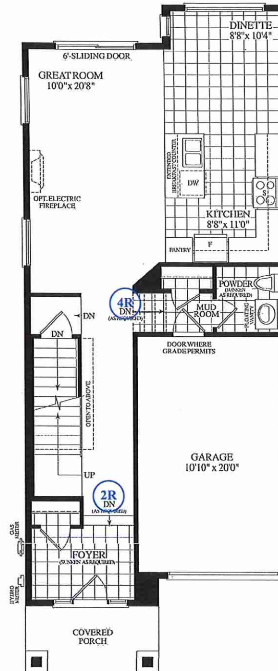
MAIN LEVEL ELEV. B
