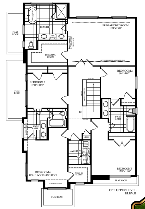
OPT. UPPER LEVEL (5 BEDROOM) ELEV. A
