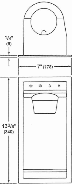
Dispenser dimensions
