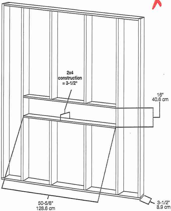
2x4 framing
