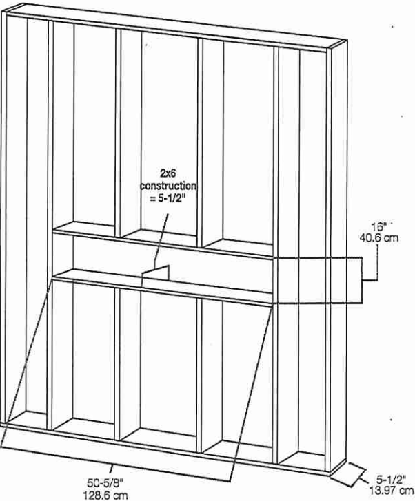
2x6 framing
