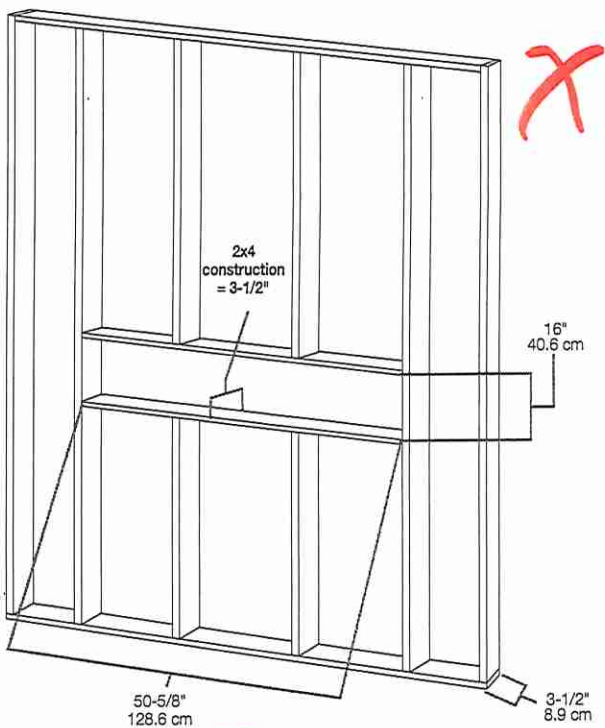
2x4 framing
