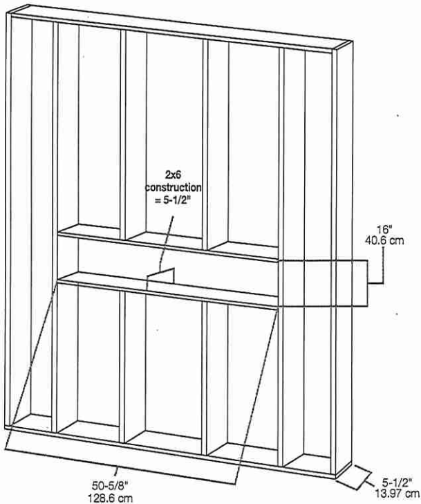
2x6 framing
