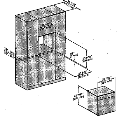
DGC7865x H7x6xBP, Einbau, 30 Zoll, Flush inset, 650S 7/8" – 22" mm – Glass, 15/16" – 23.3" mm – Stainless steel
