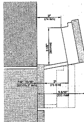
DGC 6x0x-1 + EBA 6808, DGC 6x6x (AM) + EBA 6808, DGC 7xxx(EBA 784/68) installation drawing, Proud, NA
