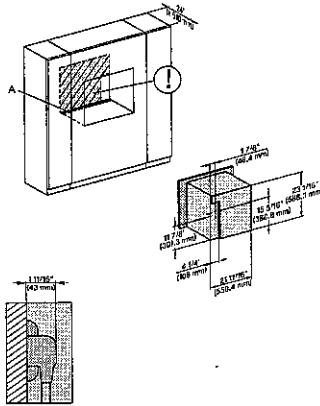
DGC7865x(+EBA7848), DGC7x8x, Installation, 30 Zoll, Proud, wide front, XXL,
