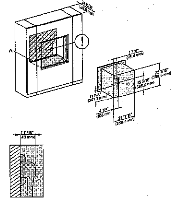
DGC7x8x(+EBA7848), Installation, 30 Zoll, Flush inset, wide front, XXL
