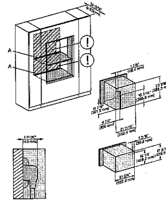
DGC786x+EBA7868, H7x40BM(+EBA7848), Installation, 30 Zoll, Flush inset, combi, wide front, XXL, 450S
