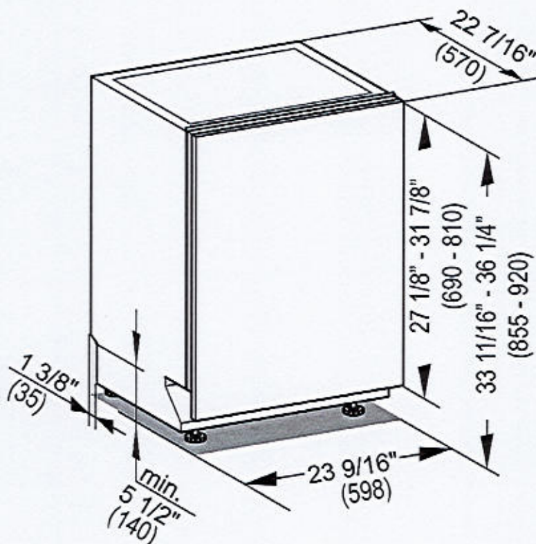
Product Dimensions
