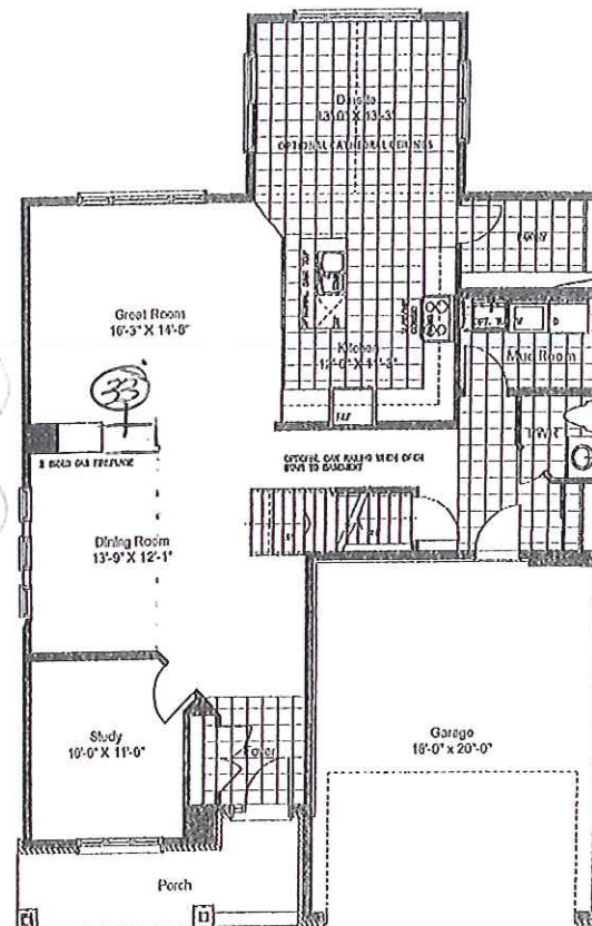
GROUND FLOOR - ELEVATION A
