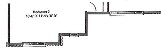
SECOND FLOOR-ELEVATION B
