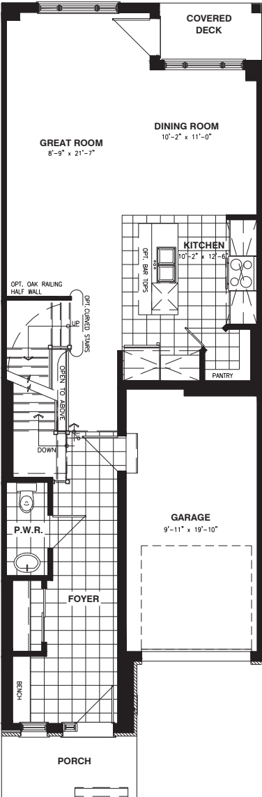
GROUND FLOOR
