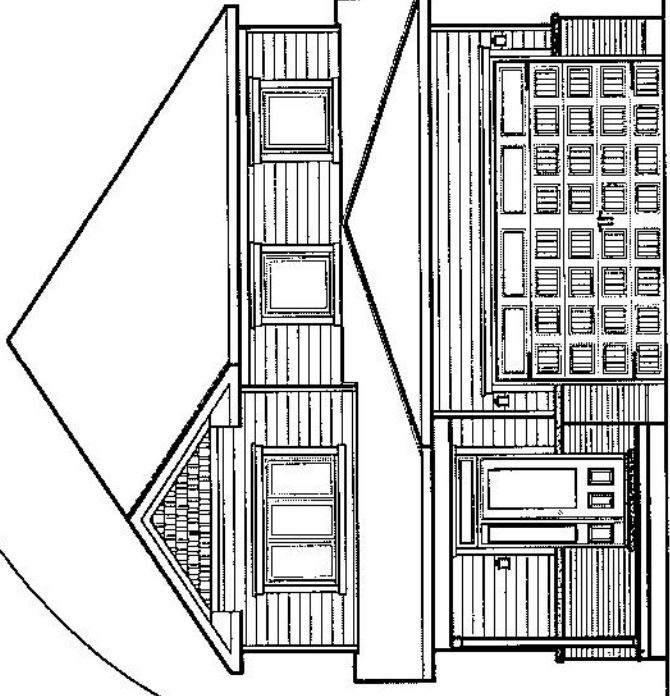
ELEVATION C
