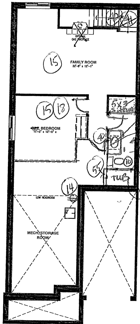
BASEMENT FLOOR
