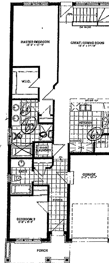
GROUND FLOOR OPTIONAL 2 BEDROOM PLAN
