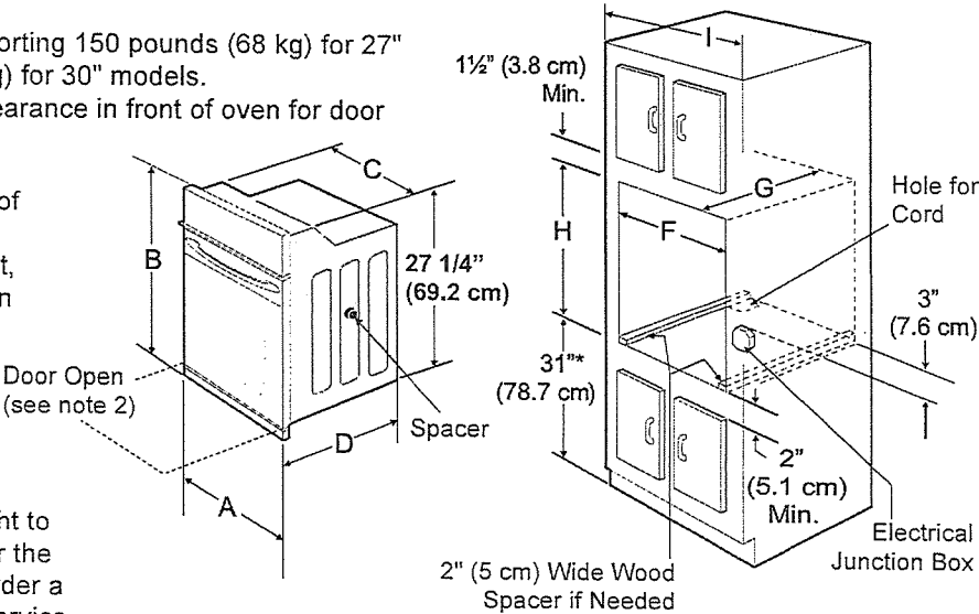
Figure 1 27" and 30" Single Wall Ovens
