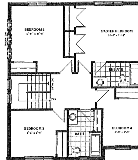
SECOND FLOOR - OPTIONAL 4 BEDROOMS ELEVATION A
