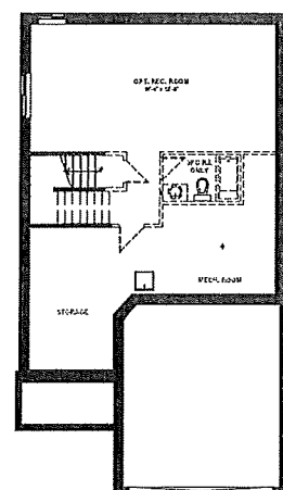
BASEMENT FLOOR
