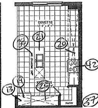
OPTIONAL KITCHEN #1
