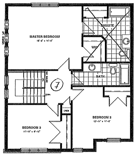
SECOND FLOOR - 3 BEDROOMS ELEVATION A
