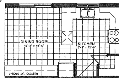
OPTIONAL KITCHEN #1
