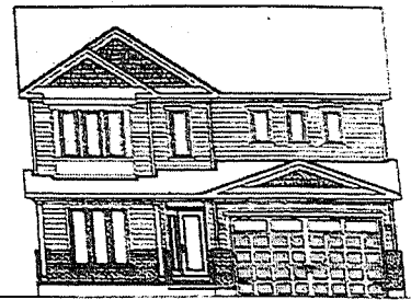
ELEVATION C
