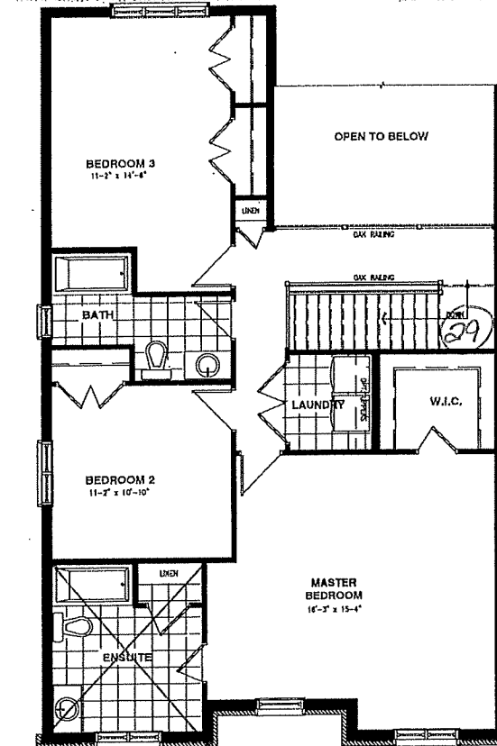
SECOND FLOOR - 3 BEDROOMS - ELEVATION A
