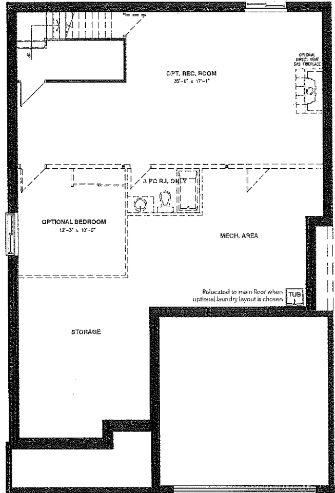
BASEMENT FLOOR - ELEVATION A & B C
