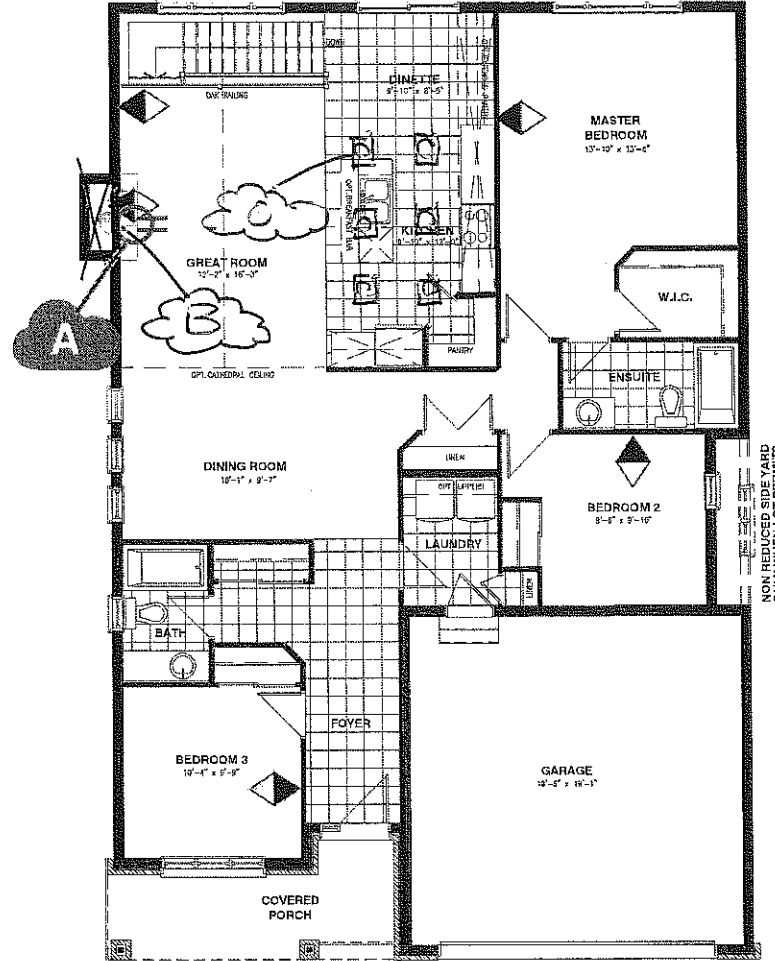
GROUND FLOOR - ELEVATION A & B C
