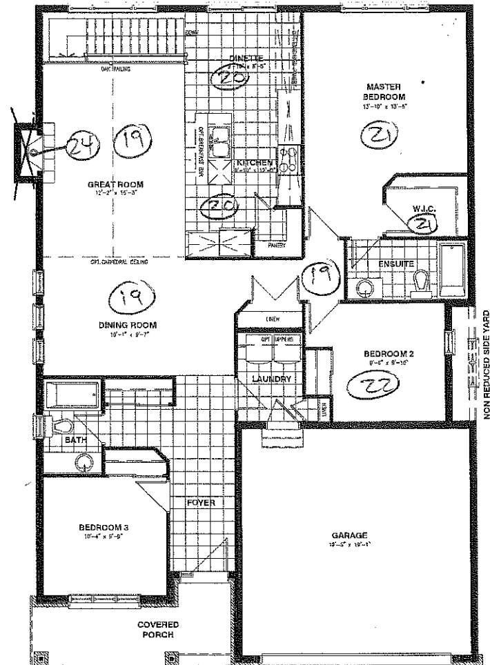
GROUND FLOOR - ELEVATION A & XC
