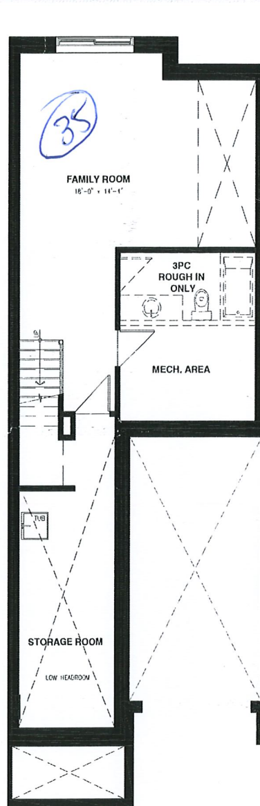
BASEMENT FLOOR
