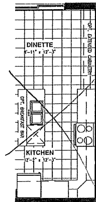
OPTIONAL KITCHEN #2
