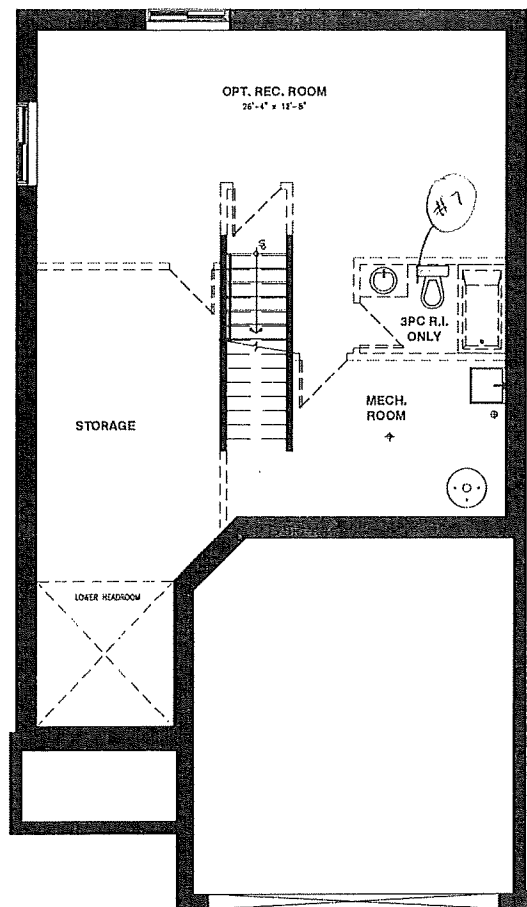
BASEMENT FLOOR
