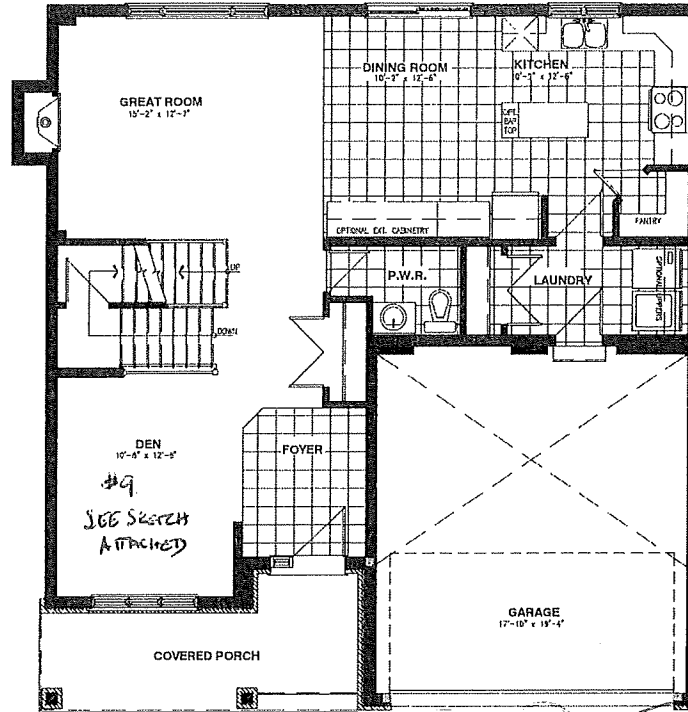
GROUND FLOOR - ELEVATION A & B
